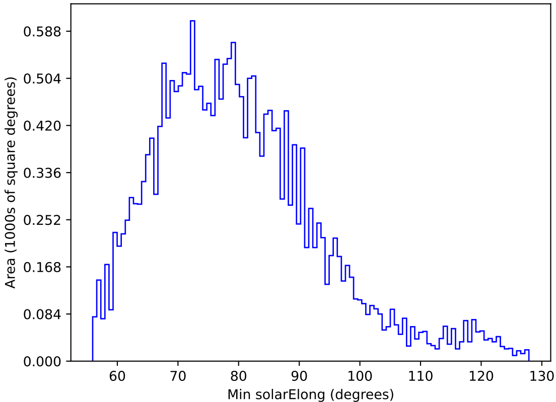
too_elab_r32_d3_griz_v3.4_10yrs All sky u band: Min solarElong
