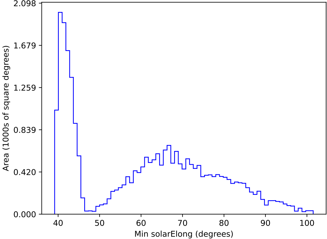
too_elab_r32_d3_griz_v3.4_10yrs All sky r band: Min solarElong
