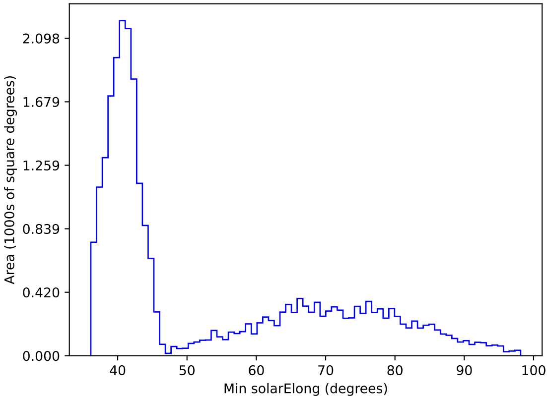
too_elab_r32_d3_griz_v3.4_10yrs All sky i band: Min solarElong
