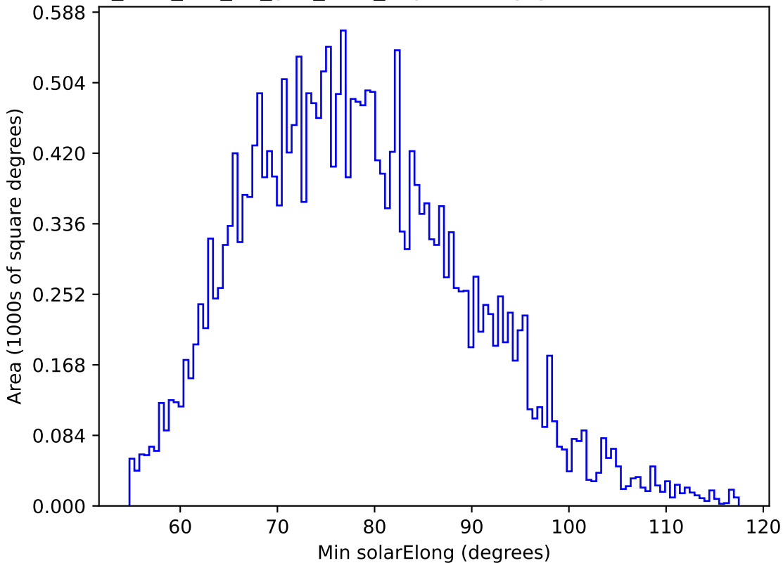
too_elab_r32_d3_griz_v3.4_10yrs All sky g band: Min solarElong
