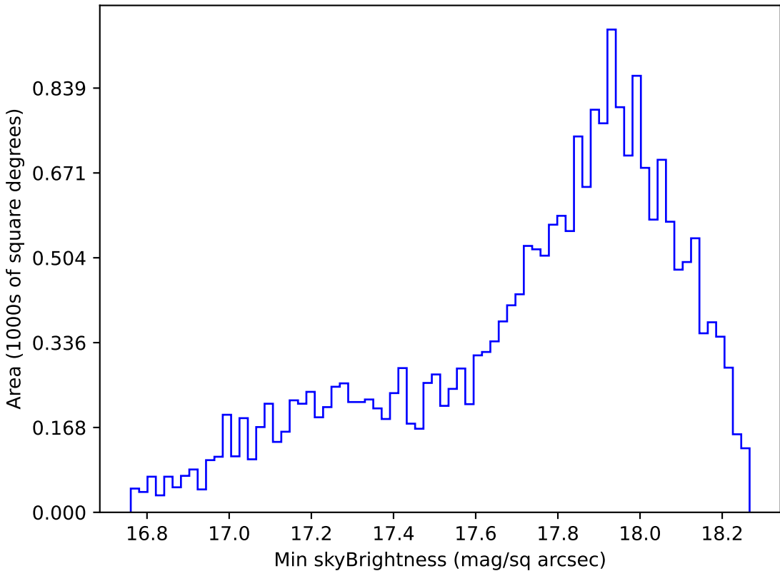
too_elab_r32_d3_griz_v3.4_10yrs Yr 1 y band: Min skyBrightness
