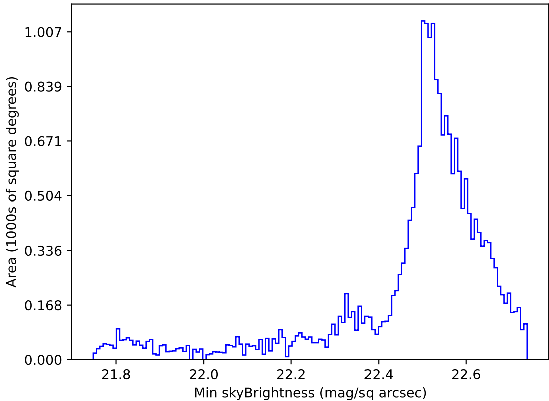
too_elab_r32_d3_griz_v3.4_10yrs Yr 1 u band: Min skyBrightness
