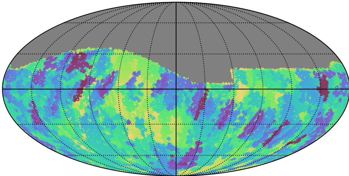
too_elab_r32_d3_griz_v3.4_10yrs Yr 1 r band: Min skyBrightness
