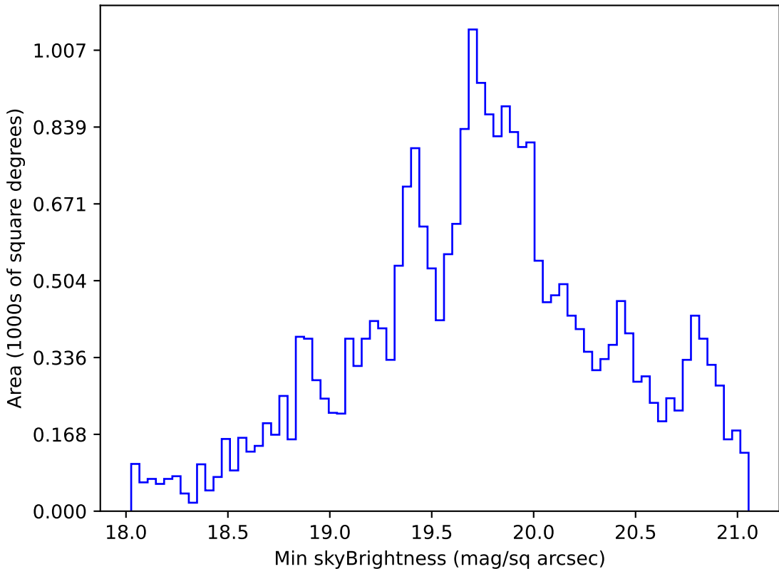
too_elab_r32_d3_griz_v3.4_10yrs Yr 1 r band: Min skyBrightness
