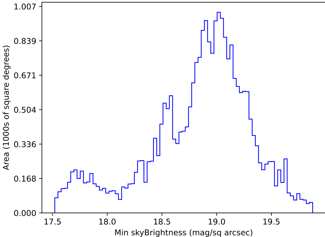
too_elab_r32_d3_griz_v3.4_10yrs Yr 1 i band: Min skyBrightness
