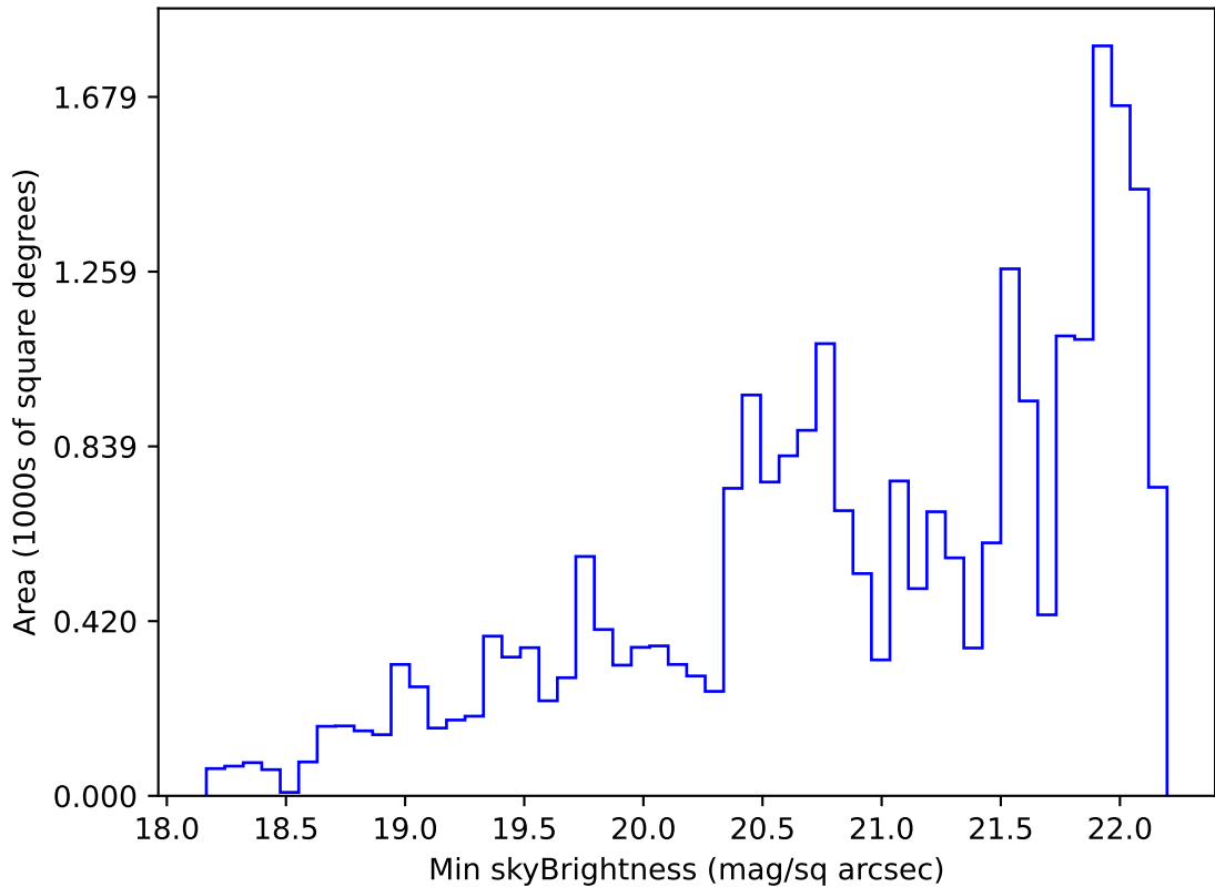
too_elab_r32_d3_griz_v3.4_10yrs Yr 1 g band: Min skyBrightness
