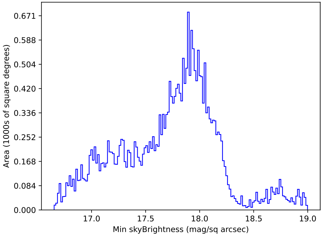
too_elab_r32_d3_griz_v3.4_10yrs Yr 1 all bands: Min skyBrightness
