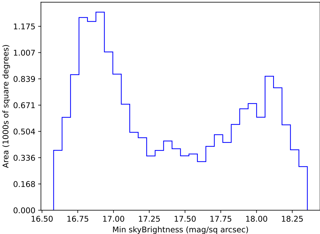
too_elab_r32_d3_griz_v3.4_10yrs WFD z band: Min skyBrightness
