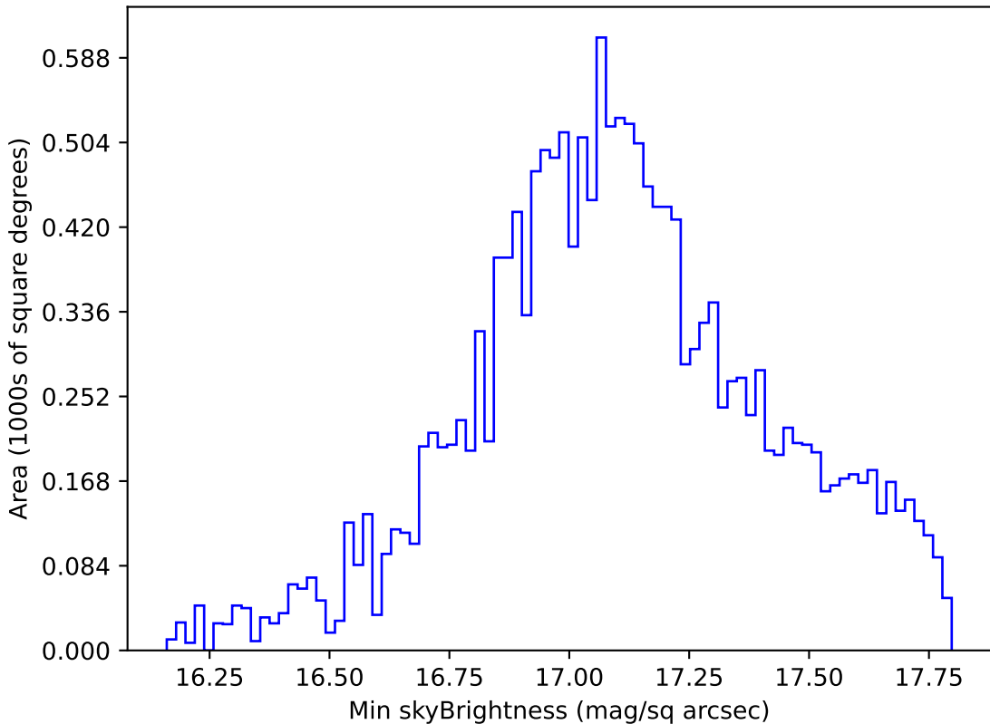
too_elab_r32_d3_griz_v3.4_10yrs WFD y band: Min skyBrightness
