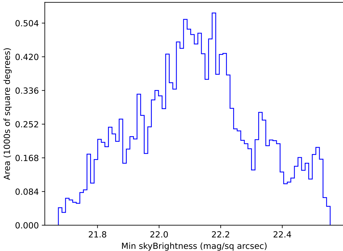
too_elab_r32_d3_griz_v3.4_10yrs WFD u band: Min skyBrightness
