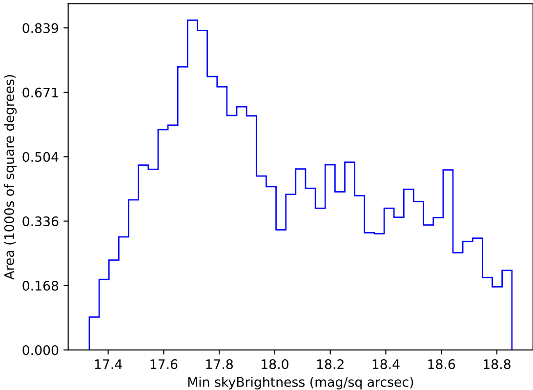
too_elab_r32_d3_griz_v3.4_10yrs WFD i band: Min skyBrightness
