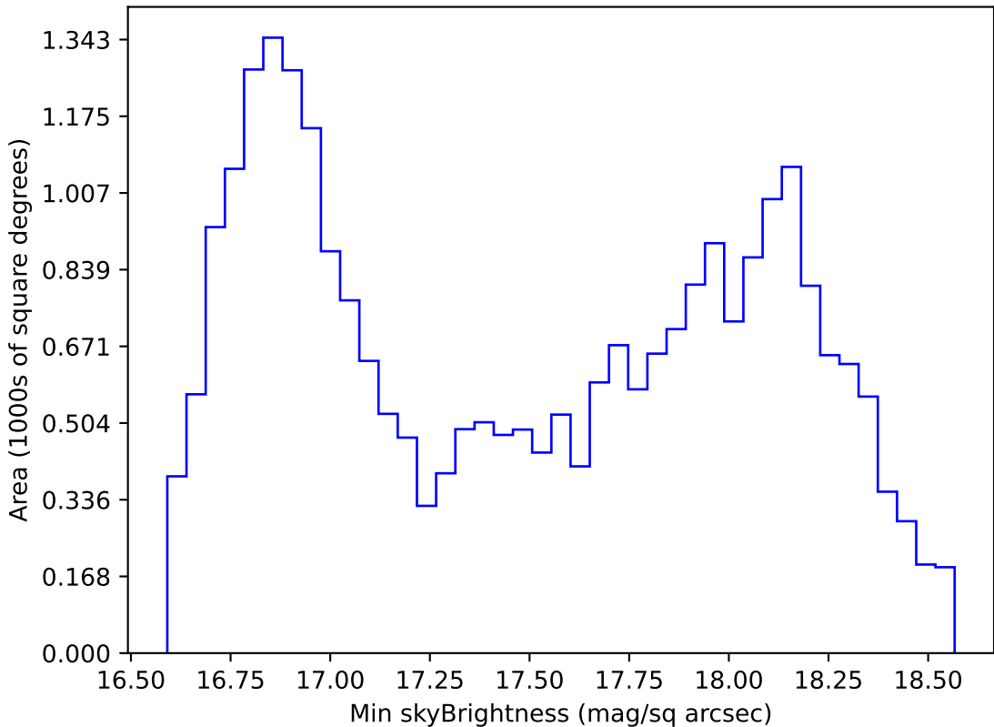
too_elab_r32_d3_griz_v3.4_10yrs All sky z band: Min skyBrightness
