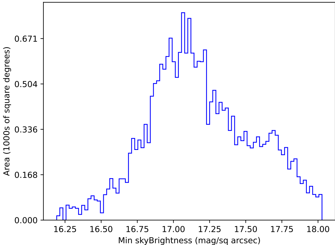
too_elab_r32_d3_griz_v3.4_10yrs All sky y band: Min skyBrightness
