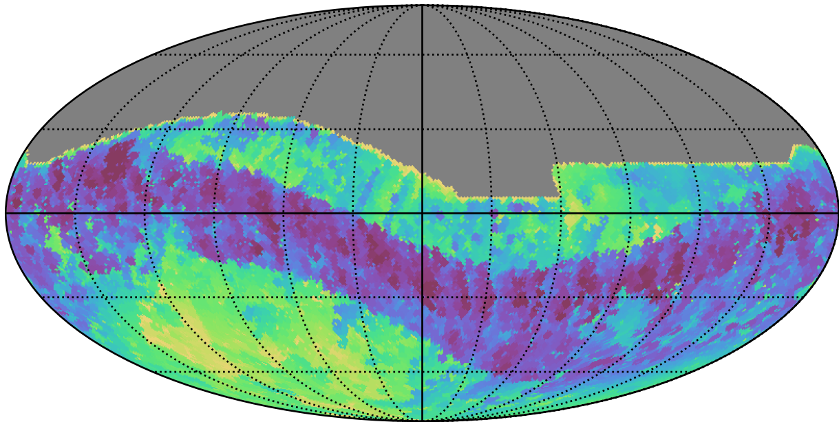
too_elab_r32_d3_griz_v3.4_10yrs All sky i band: Min skyBrightness
