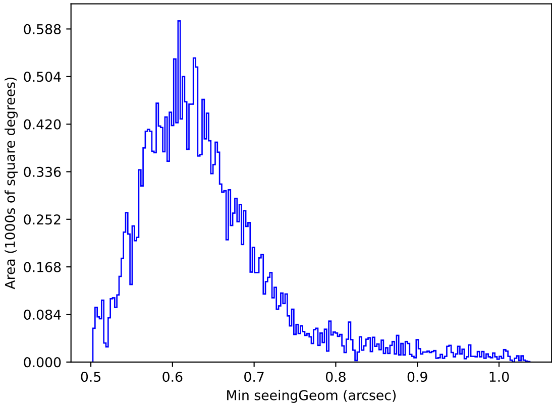
too_elab_r32_d3_griz_v3.4_10yrs Yr 1 z band: Min seeingGeom
