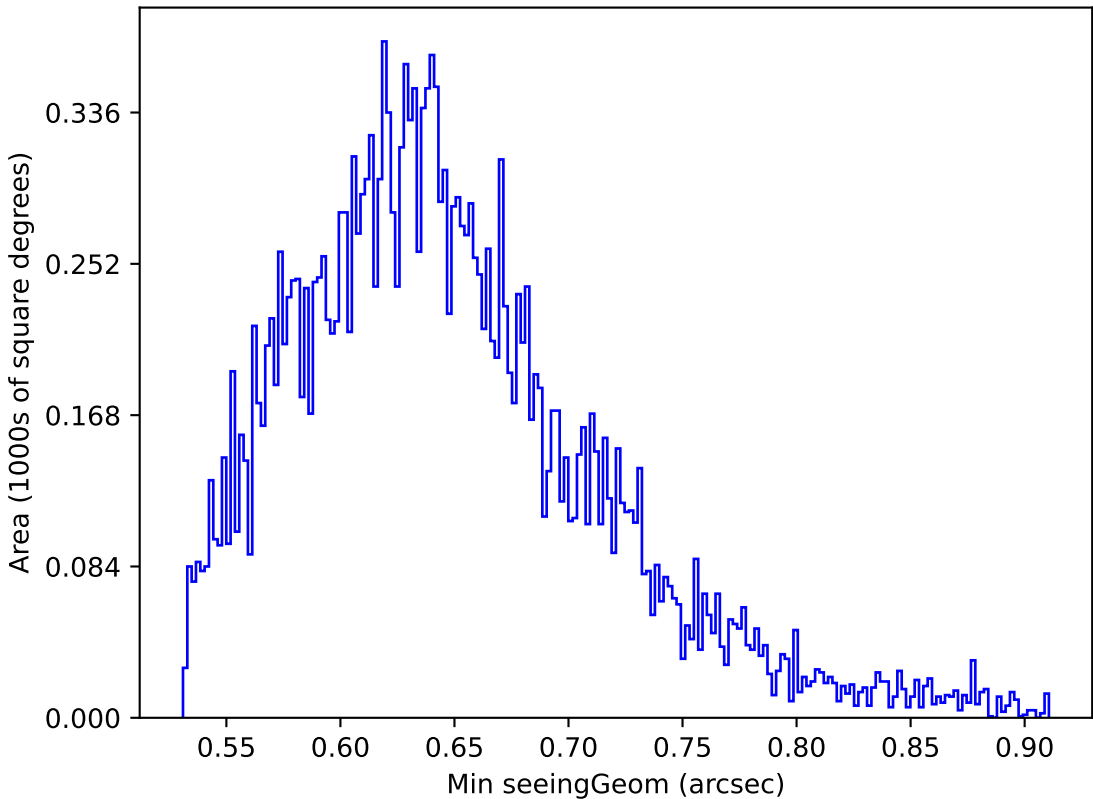
too_elab_r32_d3_griz_v3.4_10yrs Yr 1 y band: Min seeingGeom
