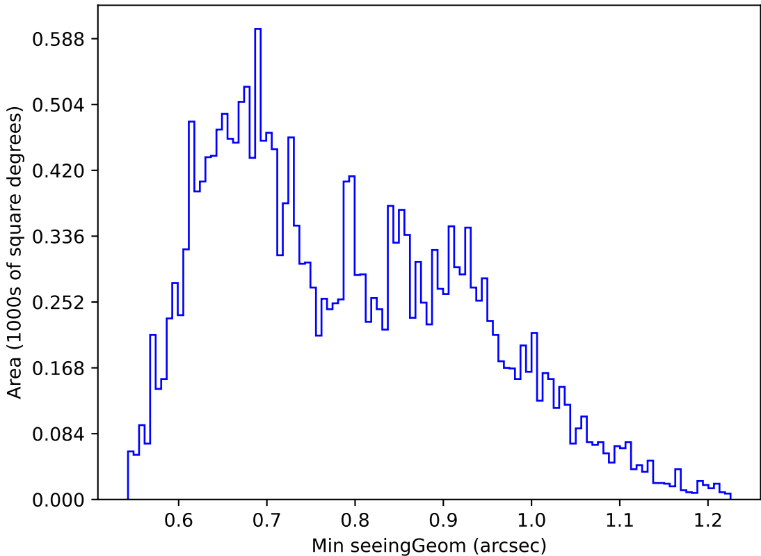
too_elab_r32_d3_griz_v3.4_10yrs Yr 1 u band: Min seeingGeom
