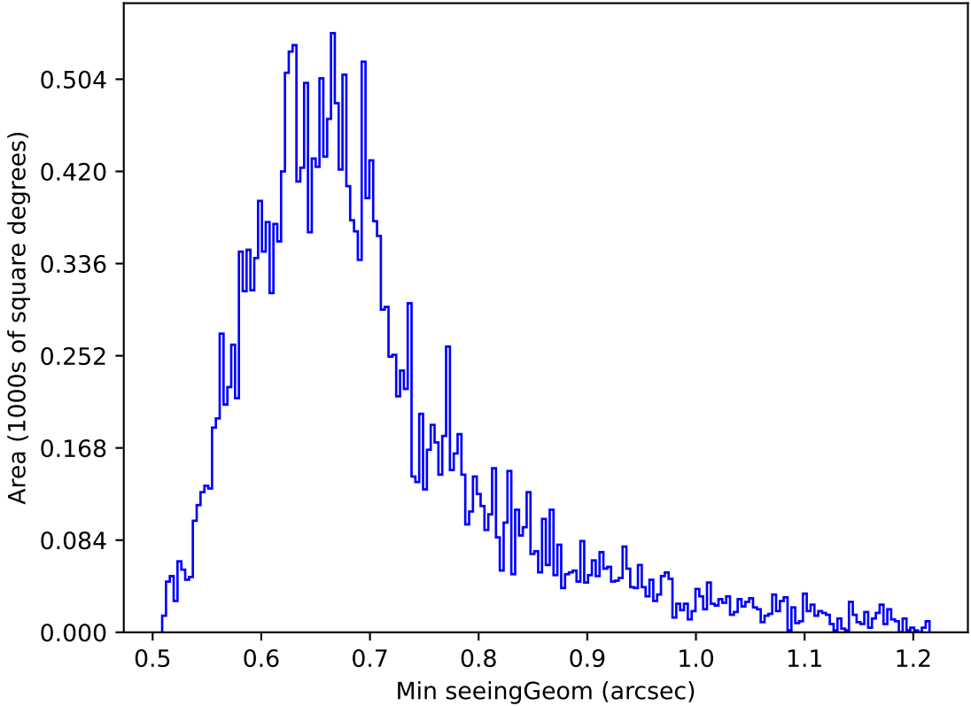
too_elab_r32_d3_griz_v3.4_10yrs Yr 1 g band: Min seeingGeom
