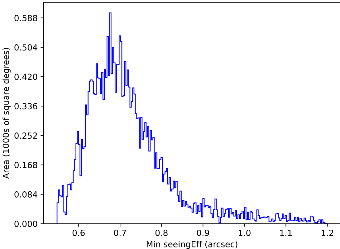
too_elab_r32_d3_griz_v3.4_10yrs Yr 1 z band: Min seeingEff
