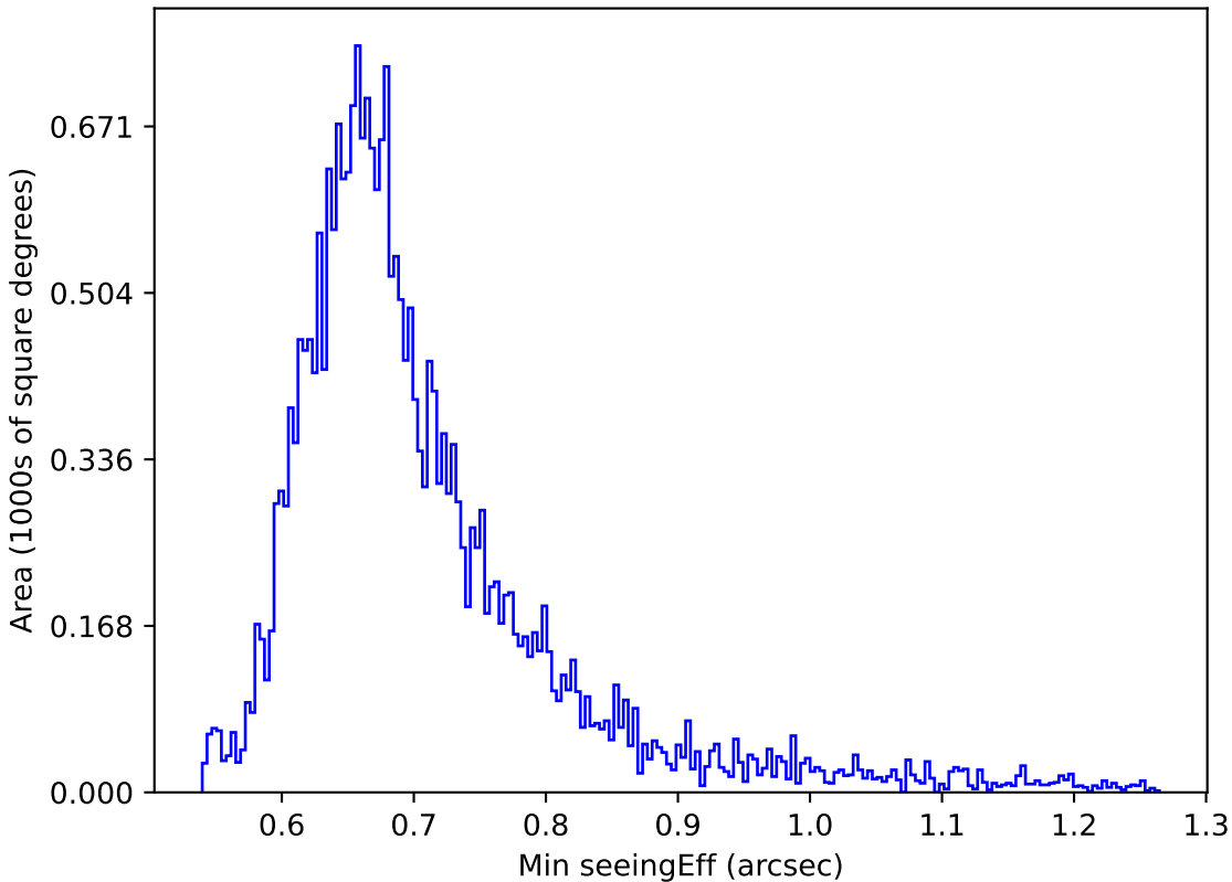
too_elab_r32_d3_griz_v3.4_10yrs Yr 1 i band: Min seeingEff
