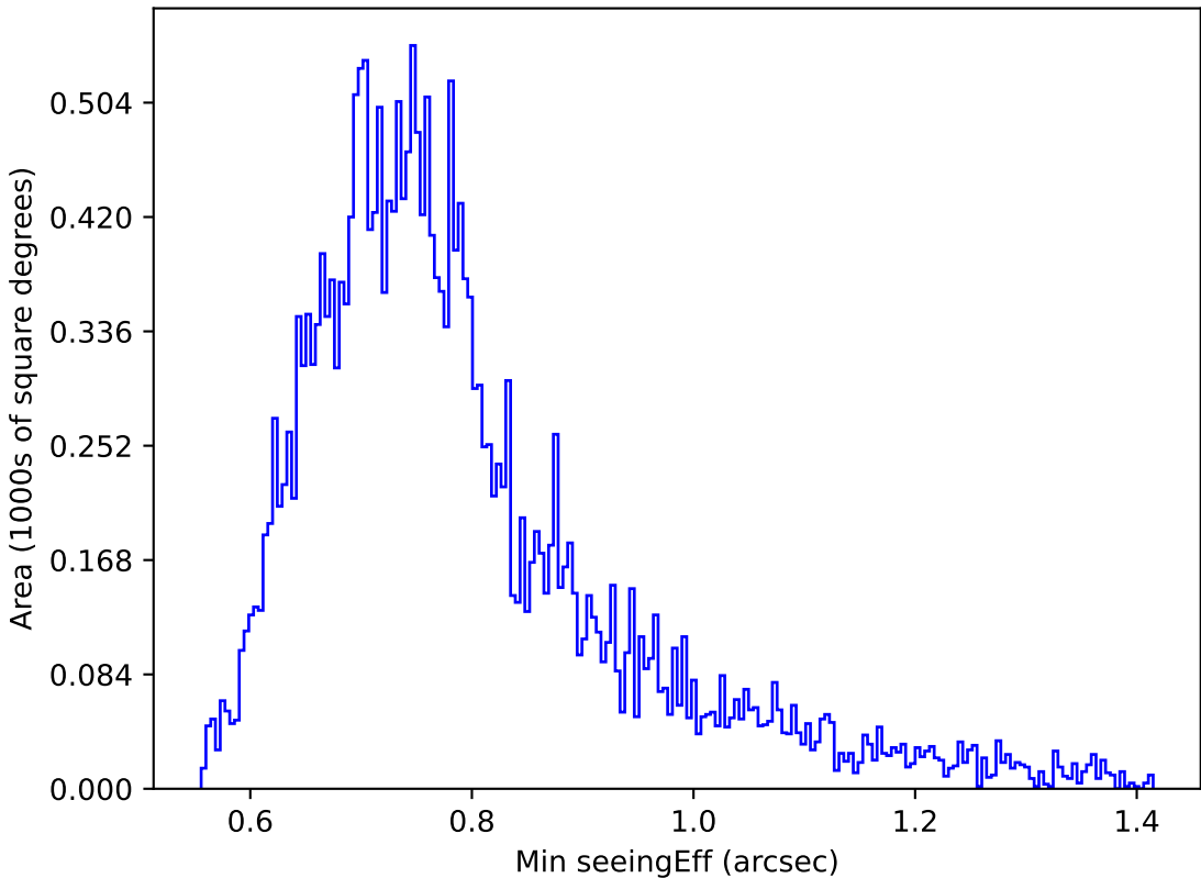
too_elab_r32_d3_griz_v3.4_10yrs Yr 1 g band: Min seeingEff
