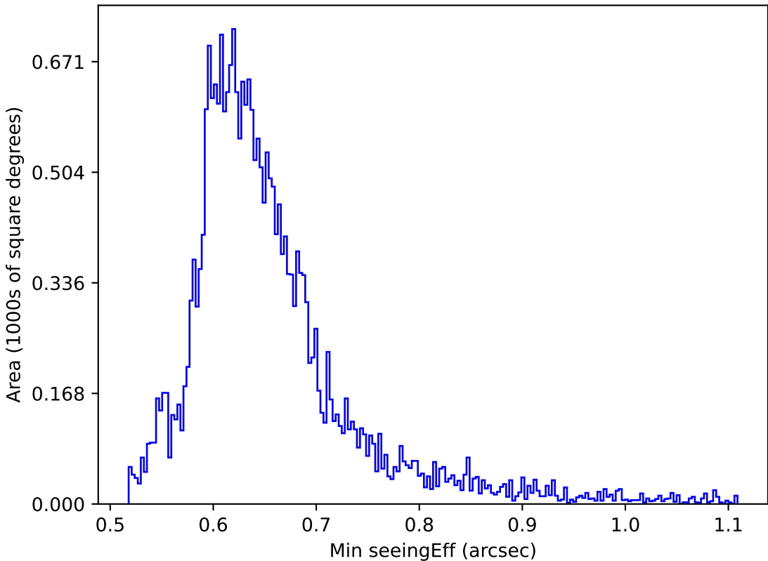
too_elab_r32_d3_griz_v3.4_10yrs Yr 1 all bands: Min seeingEff
