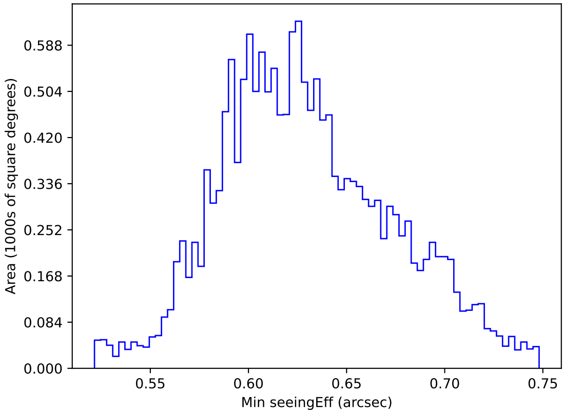
too_elab_r32_d3_griz_v3.4_10yrs WFD y band: Min seeingEff
