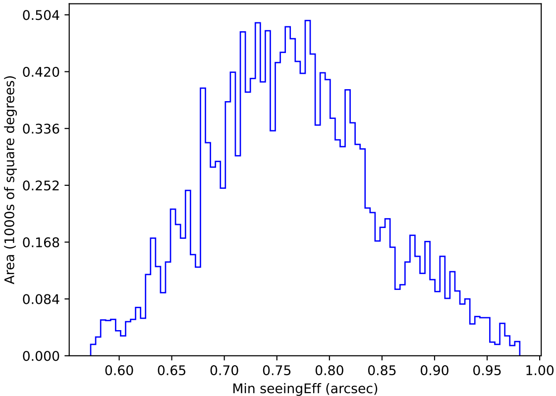
too_elab_r32_d3_griz_v3.4_10yrs WFD u band: Min seeingEff
