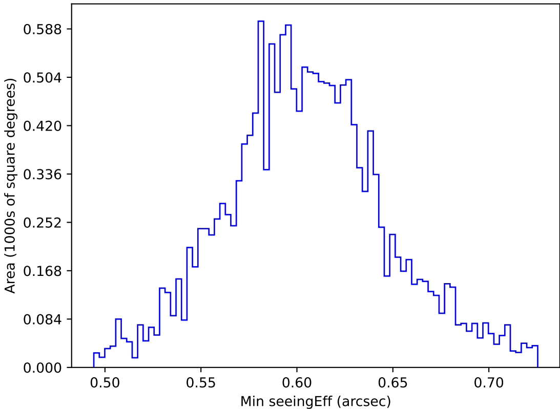
too_elab_r32_d3_griz_v3.4_10yrs WFD i band: Min seeingEff
