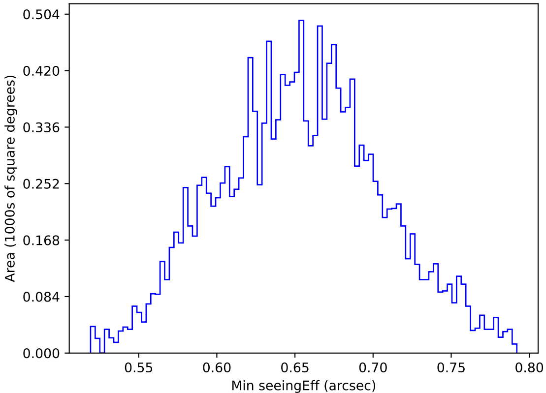
too_elab_r32_d3_griz_v3.4_10yrs WFD g band: Min seeingEff
