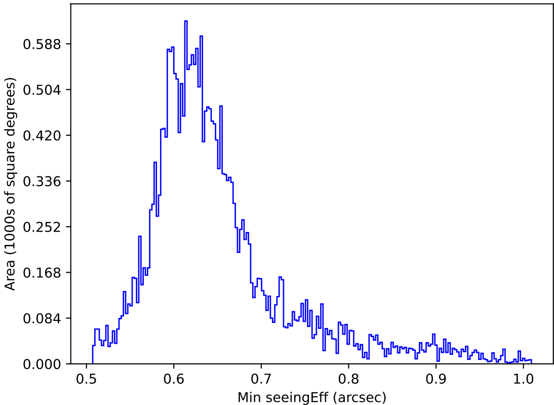
too_elab_r32_d3_griz_v3.4_10yrs All sky z band: Min seeingEff
