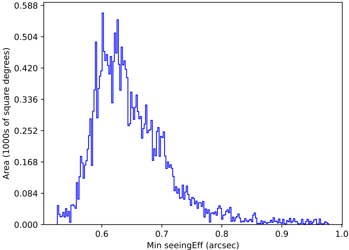
too_elab_r32_d3_griz_v3.4_10yrs All sky y band: Min seeingEff
