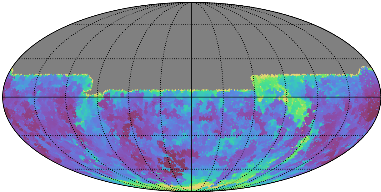
too_elab_r32_d3_griz_v3.4_10yrs All sky u band: Min seeingEff
