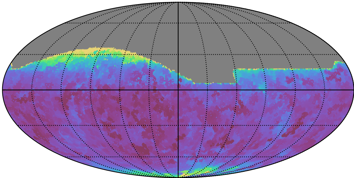
too_elab_r32_d3_griz_v3.4_10yrs All sky r band: Min seeingEff
