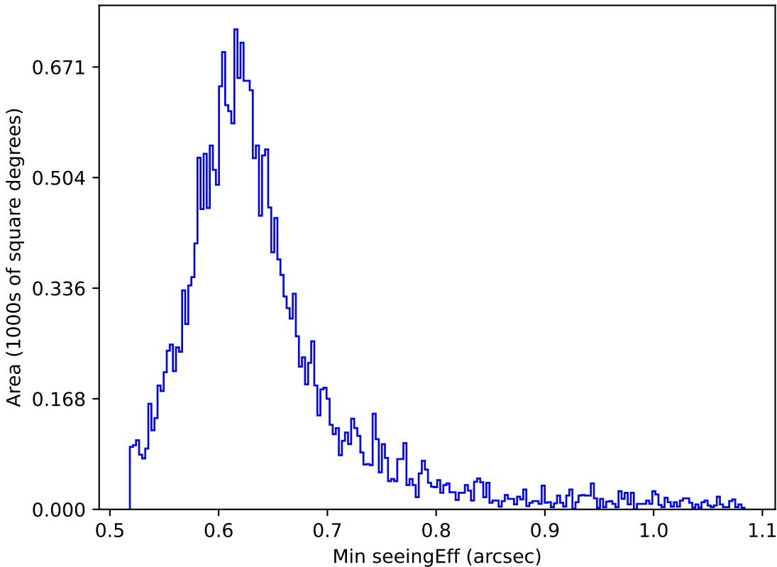
too_elab_r32_d3_griz_v3.4_10yrs All sky r band: Min seeingEff
