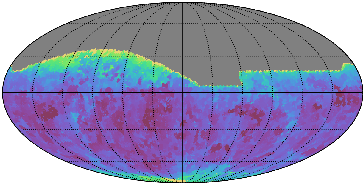
too_elab_r32_d3_griz_v3.4_10yrs All sky i band: Min seeingEff
