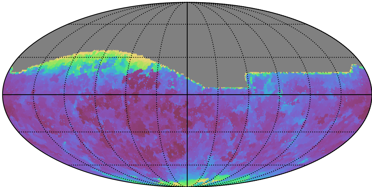
too_elab_r32_d3_griz_v3.4_10yrs All sky g band: Min seeingEff
