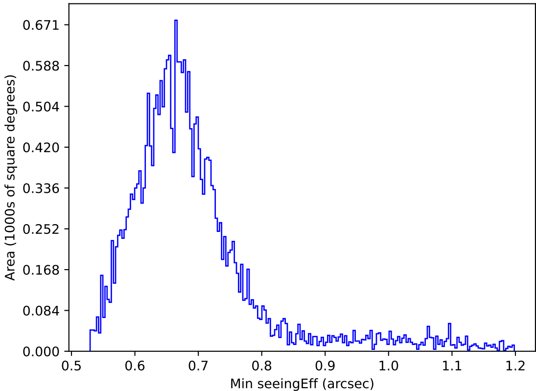
too_elab_r32_d3_griz_v3.4_10yrs All sky g band: Min seeingEff
