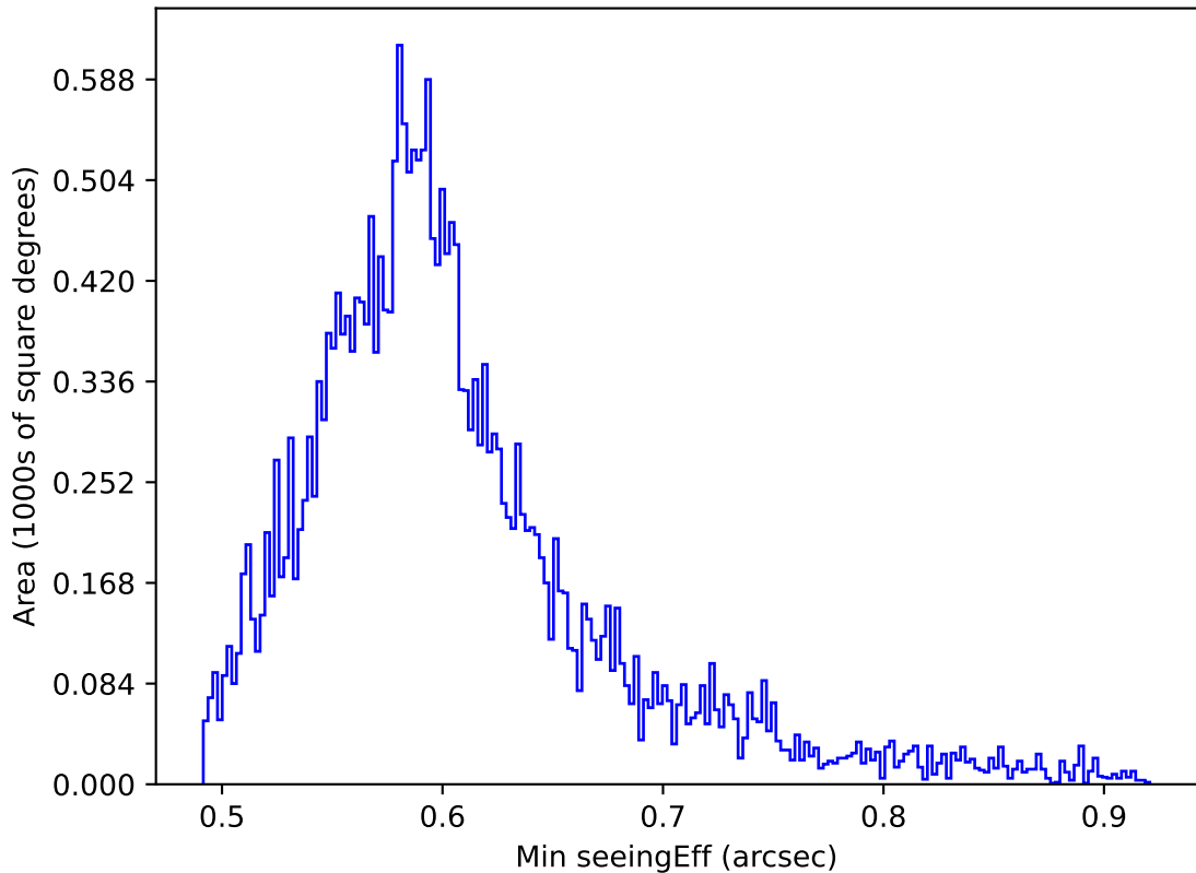
too_elab_r32_d3_griz_v3.4_10yrs All sky all bands: Min seeingEff
