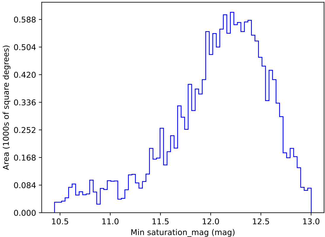
too_elab_r32_d3_griz_v3.4_10yrs WFD z band: Min saturation_mag
