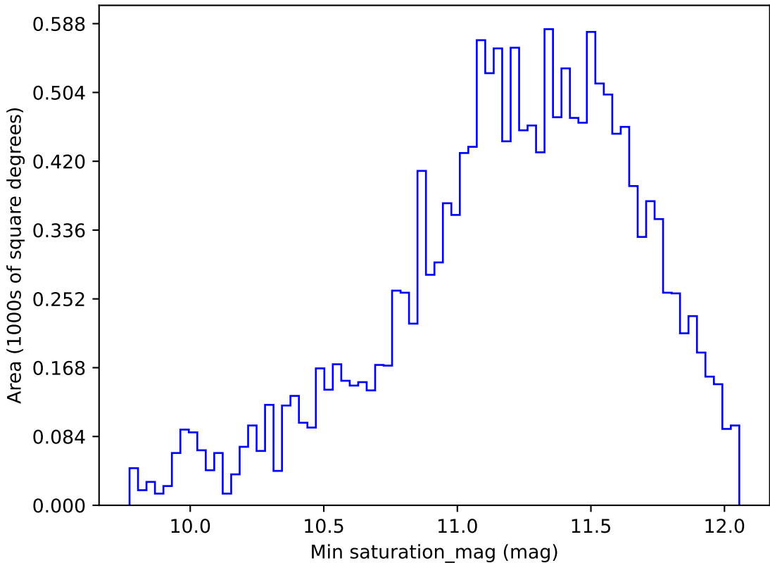
too_elab_r32_d3_griz_v3.4_10yrs WFD y band: Min saturation_mag
