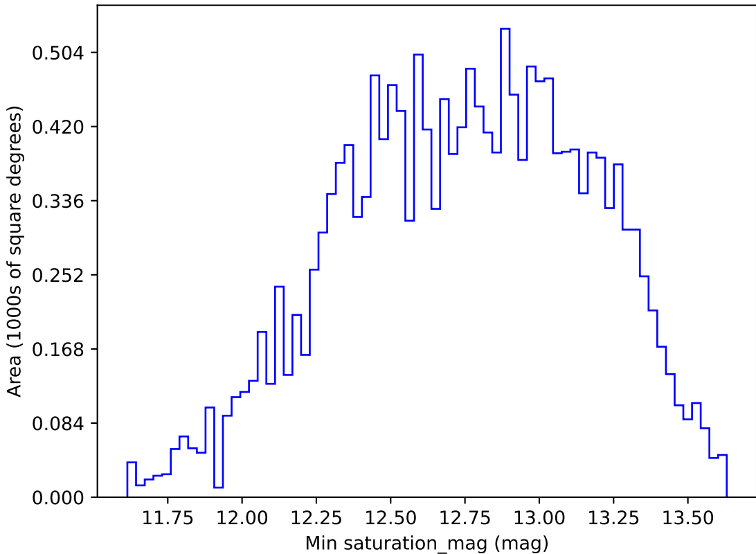
too_elab_r32_d3_griz_v3.4_10yrs WFD g band: Min saturation_mag
