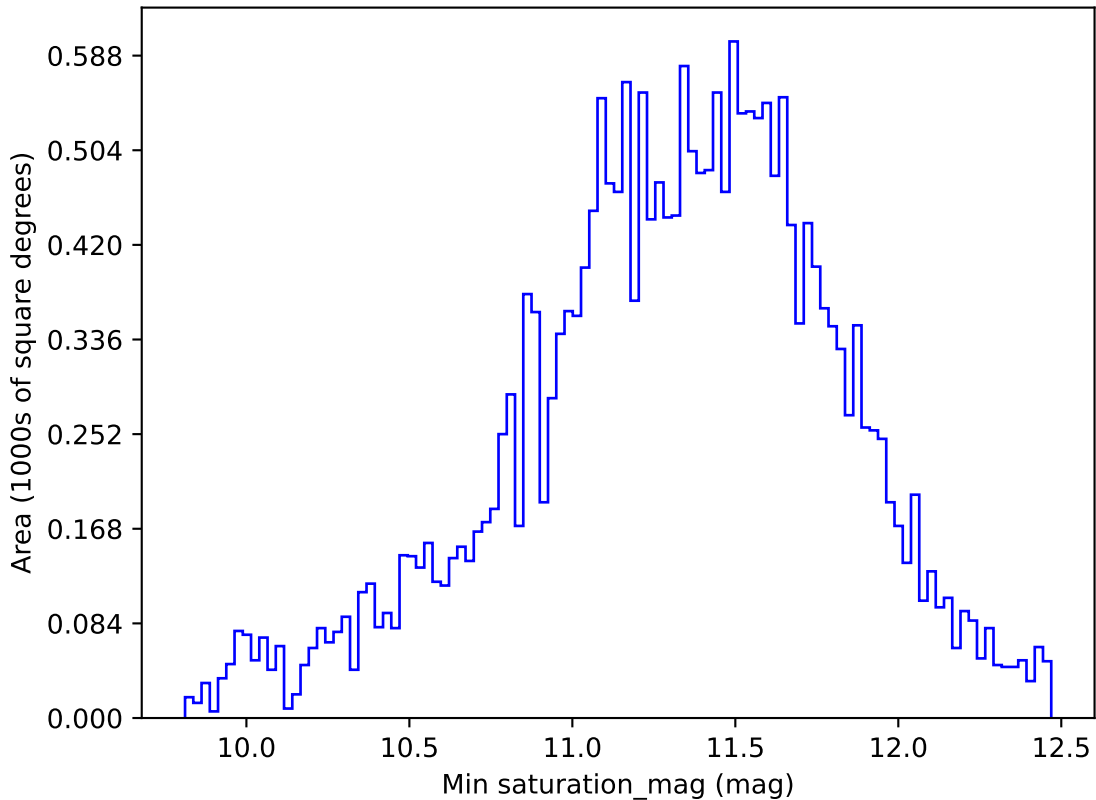
too_elab_r32_d3_griz_v3.4_10yrs All sky y band: Min saturation_mag
