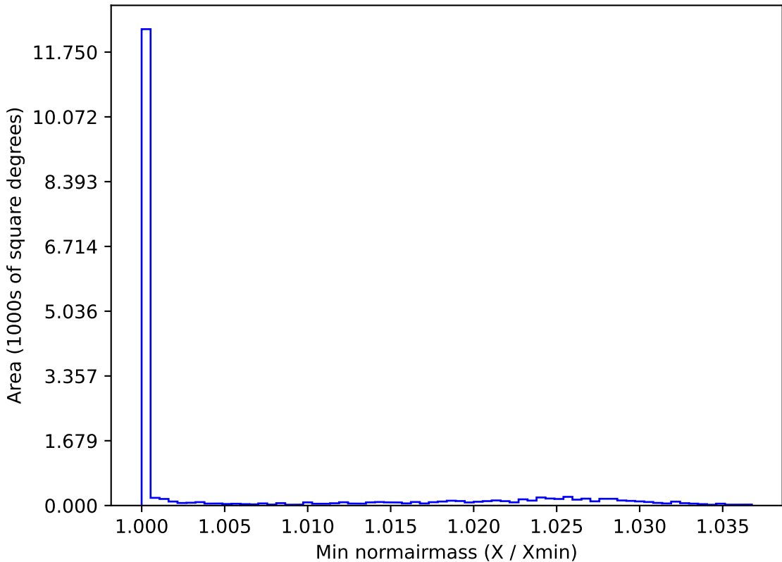
too_elab_r32_d3_griz_v3.4_10yrs WFD z band: Min normairmass
