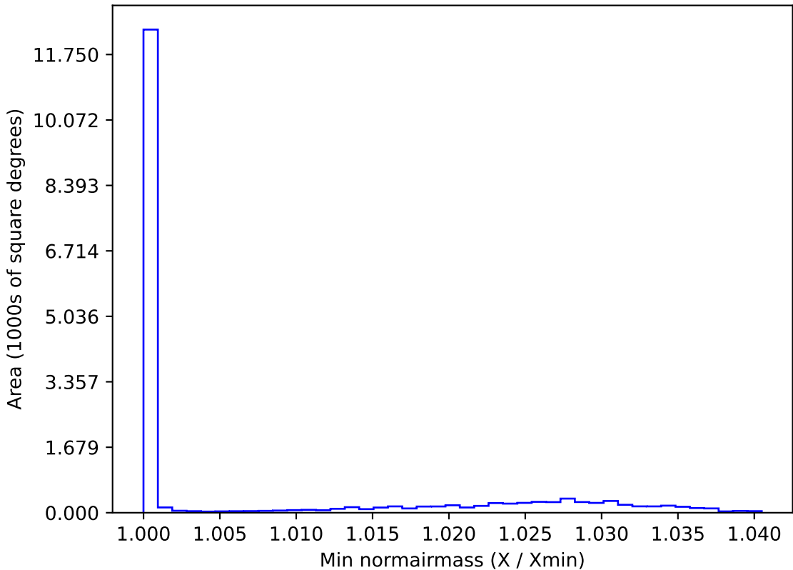
too_elab_r32_d3_griz_v3.4_10yrs WFD y band: Min normairmass
