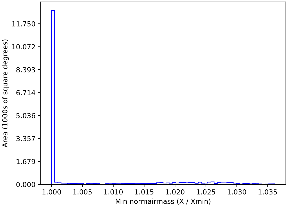
too_elab_r32_d3_griz_v3.4_10yrs WFD r band: Min normairmass
