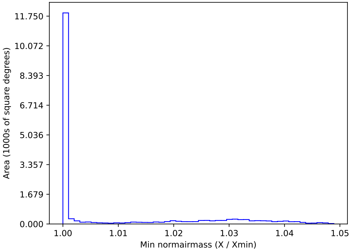
too_elab_r32_d3_griz_v3.4_10yrs WFD g band: Min normairmass
