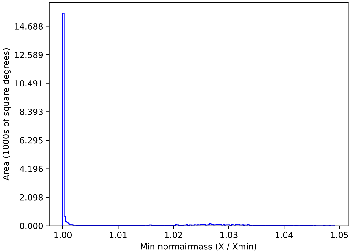
too_elab_r32_d3_griz_v3.4_10yrs All sky y band: Min normairmass
