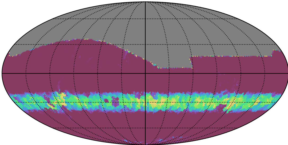
too_elab_r32_d3_griz_v3.4_10yrs All sky r band: Min normairmass
