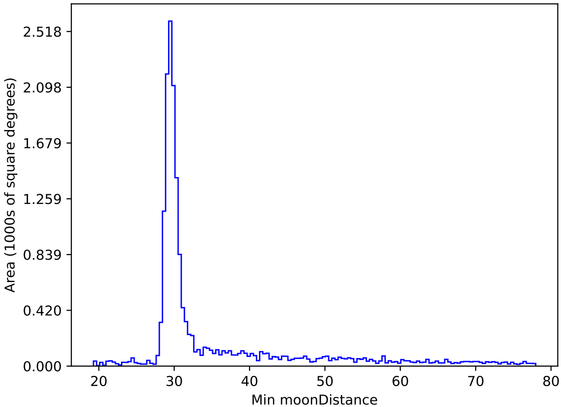
too_elab_r32_d3_griz_v3.4_10yrs WFD z band: Min moonDistance
